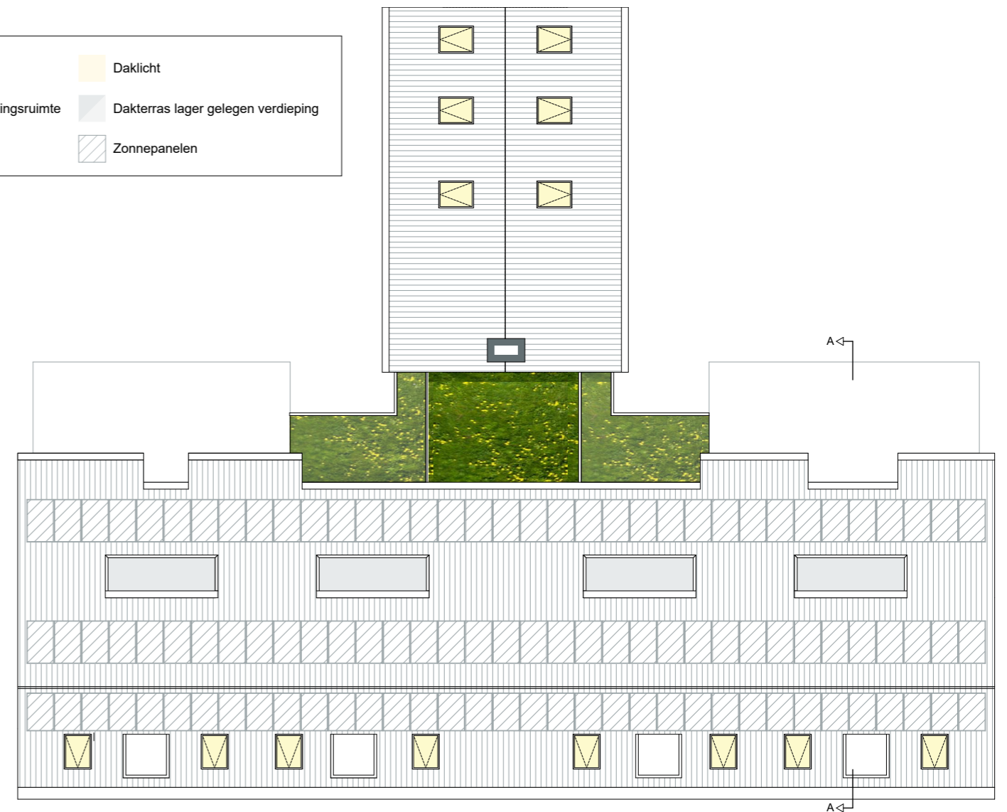
Dak (+14450)
