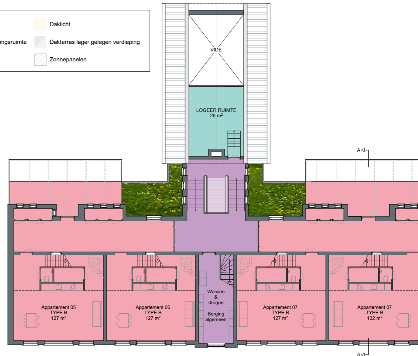
Verdieping 1 (+4990)
